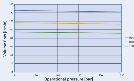
Volume flow
