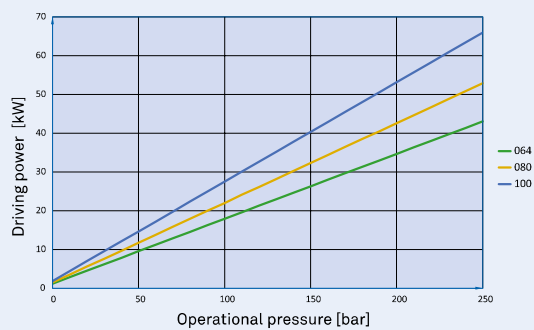
Driving power
